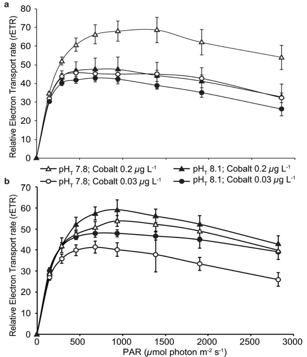
Fig 3. Relative electron transport rate (rETR) versus irradiance (PAR) for colonies of Stylophora pistillata (a) and Acropora muricata (b) (mean \pm SD, n = 10 ) exposed during five weeks to two \text{pH}_T conditions ( \text{pH}_T 7.8 or 8.1) and two cobalt concentrations (Natural and Polluted).
